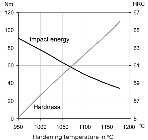
Original dimension 9 x 12 mm Tempering 3 x 1 hour at 560° C Unnotched test piece 7 x 10 x 55 mm
