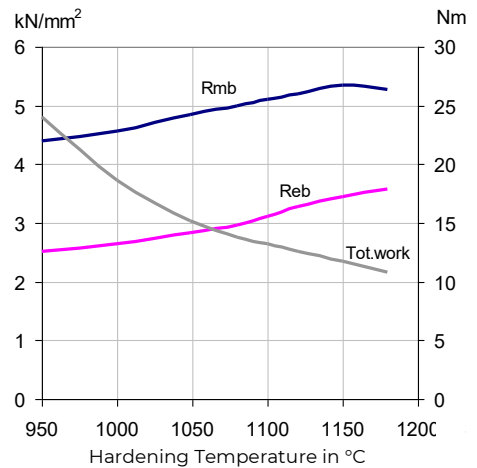
Original dimension Ø 6 mm Tempering 3 x 1 hour at 560°C Dimension of test piece Ø 4.7 mm Rmb = Ultimate bend strength in kN/mm 2 Reb = Bend yield strength in kN/mm 2 Tot. work = Total work in Nm
